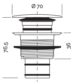
Válvula clic-clac cromo (mm)
