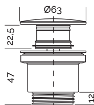
Válvula clic-clac Akron (mm)
