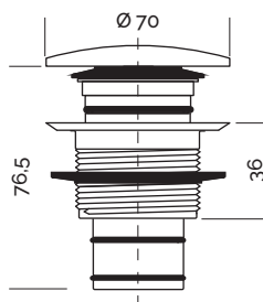
Válvula clic-clac Akron (mm)
