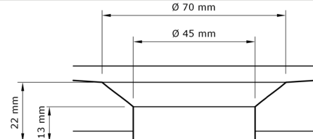
DRAINING ZONE DETAIL
